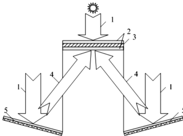
Figure 1. Principal scheme of solar collector with reflectors: 1 – falling sun rays, 2 – collector cover (glass), 3 – absorber, 4 – reflection sun rays, 5 – reflectors
