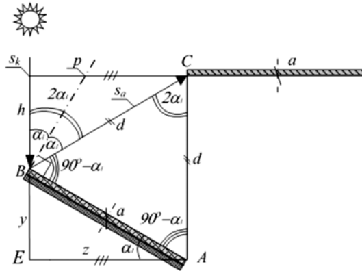
Figure 2. Detection scheme for left mirror rotation angle \alpha_1
