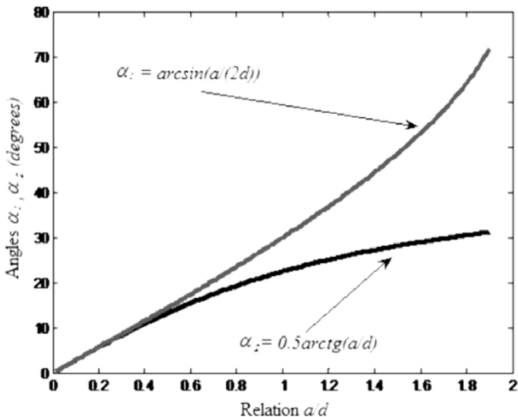
Figure 4. Dependence of right side and left side mirror angles
