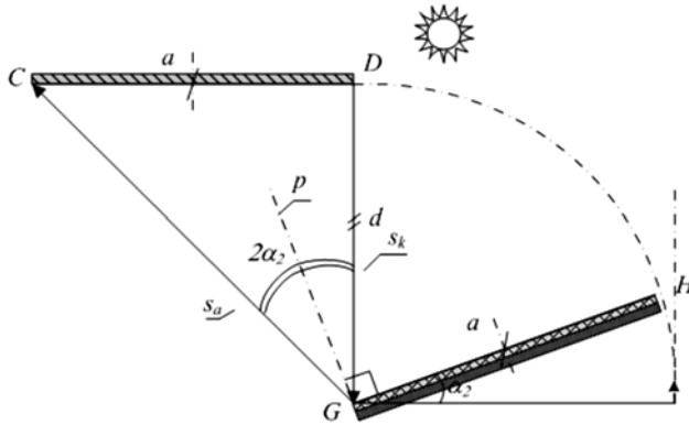
Figure 3. Detection scheme for right mirror rotation angle \alpha_2
